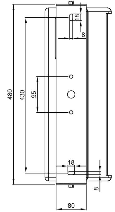
MEASURES FOR WALL ASSEMBLY
